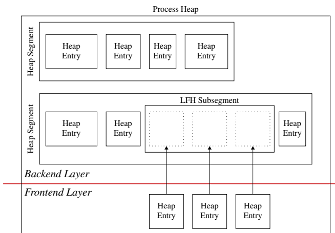
Figure 2: Simplified Windows NT heap architecture. The backend layer manages segment allocation, while the frontend layer (LFH) organizes uniformly sized allocations within subsegments.
