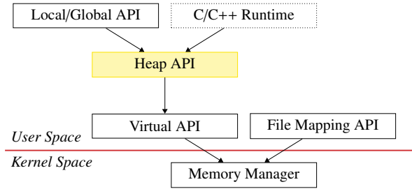
Figure 1: Windows memory management APIs available to user-space applications (Yosifovich et al., 2017).
