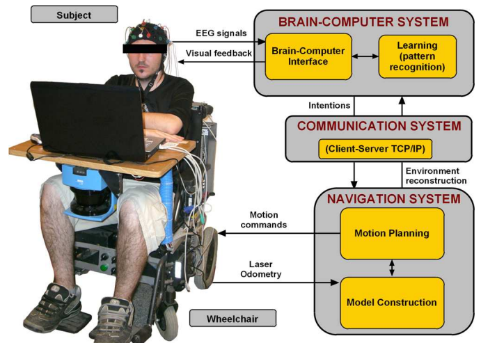
Fig. 1. Mechatronic design of the brain-actuated wheelchair, the main modules and information flow.
