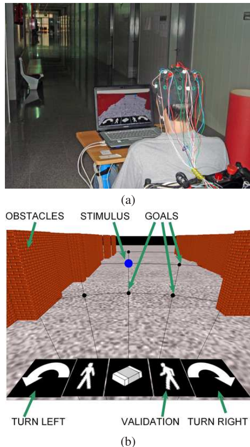
Fig. 3. (a) A snapshot of a participant navigating along a corridor. (b) Information represented in the visual display, which is an environment abstraction displayed from the user's point of view.
