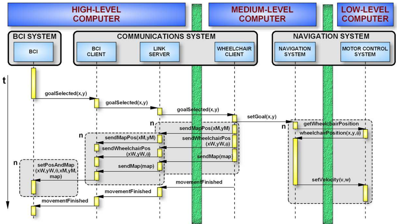
Fig. 5. The first row represents the computer hardware, whereas the second row represents the logical components. An event trace of the three integrated and running computers is shown below, illustrating a typical flow of information, starting when the user selected a destination. The flow of information and its direction are illustrated by arrows. Vertically, time increases downwards, and the vertical rectangles below the boxes represent a code execution. The dark boxes enveloping certain portions of code represent an iterative execution task.
