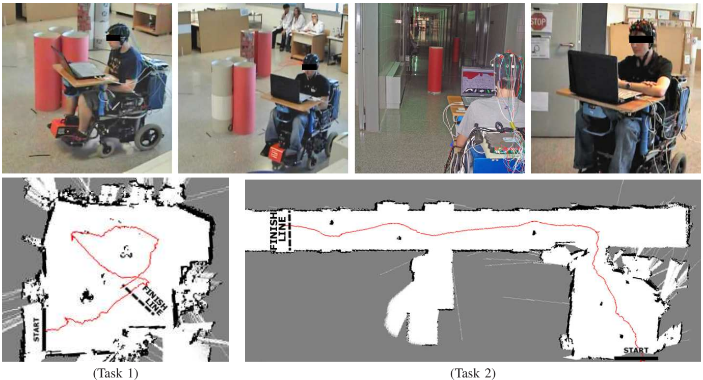
Fig. 7. The first row shows snapshots of the experiments with the wheelchair. The first two figures correspond with Task 1, and the following two figures with Task 2. The second row shows the map generated by the autonomous navigation system and the trajectory of the wheelchair in one real experiment of each task. Black zones indicate obstacles, white zones indicate known areas, and gray zones indicate unknown areas.
