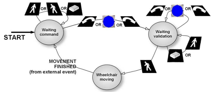
Fig. 4. Finite state machine that models the execution protocol of the options displayed on the screen to command the wheelchair.
