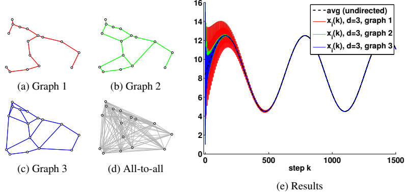
Figure 9: Sparse communication graphs. (a) Graph 1 is a Minimum-distance Spanning Tree (MST). (b) Graph 2 contains all the edges in Graph 1, and some additional links. (c) Graph 3 is more connected than Graph 2. (d) Graph with all-to-all connections. (e) Results of the proposed consensus with delay compensation for the sparse graphs in Fig. 9 (a), (b), (c). The states of each agent i = 1, \dots, n along the iterations k (abscissa-axis), for the different graphs, are shown in different colors. The average r_{avg}(k) , of the time-varying reference signals in (3) are displayed in black dashed.
