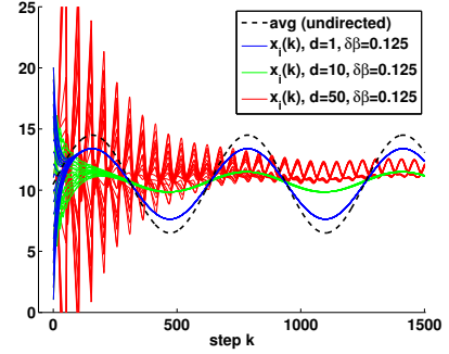
Figure 10: Dynamic consensus without delay compensation for the simulated case (S1) in Fig. 4(a) under the undirected communication graph (Fig. 3(b)). In these simulations, the delay d only affects the neighbors' states, but not the local state of agents. The states of each agent i = 1, \dots, n (solid, different colors), along the iterations k (abscissa-axis), are here depicted, together with the average of the time-varying reference signals (black dashed).
