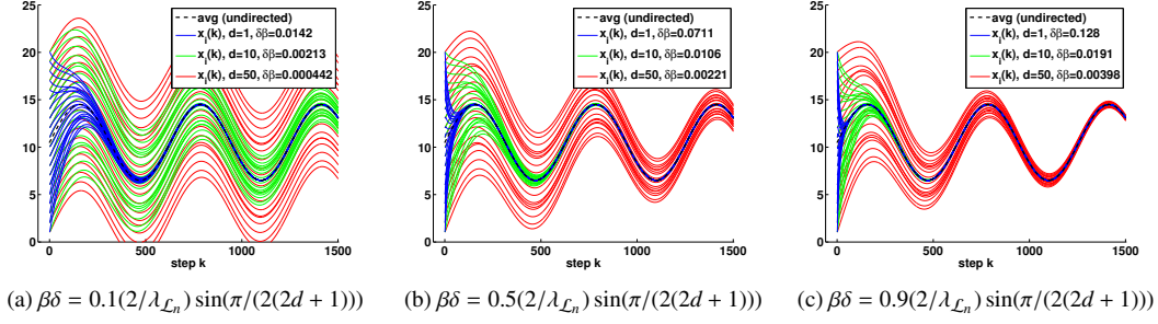
Figure 7: Alternative execution. Instead of using the proposed dynamic consensus with delay compensation [1, 2, 30], (7), for the simulated case (S1) in Fig. 4(a) under the undirected communication graph (Fig. 3(b)). The states of each agent i = 1, \dots, n (solid, different colors), along the iterations k (abscissa-axis), are here depicted, together with the average of the time-varying reference signals (black dashed).
