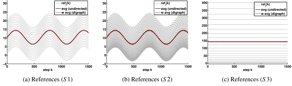
Figure 4: References measured by the robots (gray solid), along the iterations k (abscissa-axis). The weighted average r_{wavg}(k) and average r_{avg}(k) of the reference signals given by (2) and (3) are shown respectively in red solid and in black solid. These average values are associated with, respectively, the directed strongly connected and the undirected connected graphs in Fig. 3.
