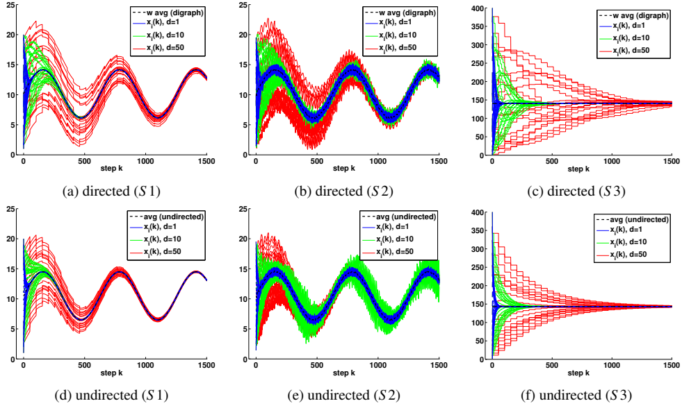
Figure 5: Proposed dynamic consensus with delay compensation for the cases (S1, S2, S3) in Fig. 4, under the directed ((a),(b),(c)) and the undirected communication graphs ((d), (e), (f)) in Fig. 3. The states of each agent i = 1, \dots, n along the iterations k (abscissa-axis), for different delay values d \in \{1, 10, 50\} are shown in different colors. The weighted average r_{wavg}(k) (directed graph: (a), (b), (c)) and the average r_{avg}(k) (undirected graph: (d), (e), (f)), of the time-varying reference signals in (2) and (3) are displayed in black dashed.
