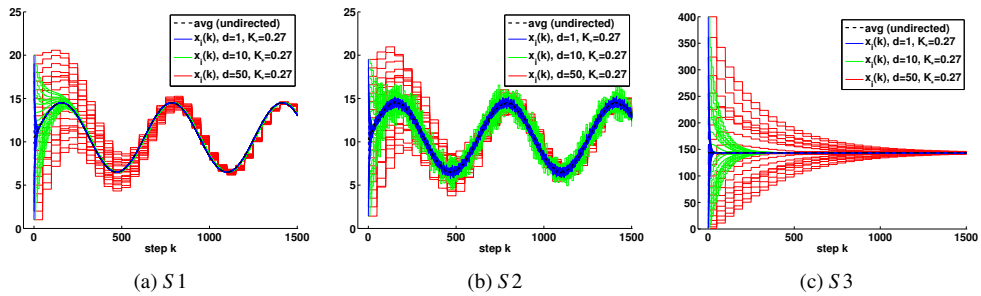
Figure 6: Alternative execution. Instead of using the proposed dynamic consensus with delay compensation, agents use here a dynamic consensus method without delay compensation [1, 2, 30], (7). Here, as discussed in Section 2.2, agents use a larger period for trying to get rid of the delay d , for the cases (S1, S2, S3) in Fig. 4 under the undirected communication graph (Fig. 3(b)). The states of each agent i = 1, \dots, n , along the iterations k (abscissa-axis), are here depicted for different delay values d \in \{1, 10, 50\} in different colors.
