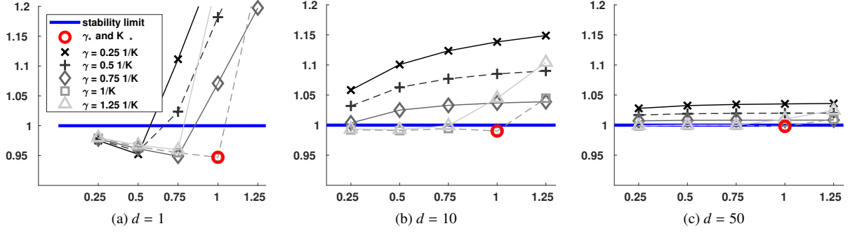
Figure 8: Convergence speed when the delay equals d = 1 (a), d = 10 (b) and d = 50 (c) for the communication graph in Figure 3(b), which is undirected. The figures contain the graphical representation of the values shown in Table 1. They represent the modulus of the leading eigenvalue. Values closer to 0 provide faster convergence speed. Values larger than one (stability limit, in blue), are associated with unstable systems. The abscissa-axis represents different values of K , which are equal to K = \text{factor}_K K_* , where \text{factor}_K \in \{0.25, 0.5, 0.75, 1, 1.25\} . Every plot represents a value of \gamma equal to \gamma = \frac{\text{factor}_\gamma}{K} , where \text{factor}_\gamma \in \{0.25, 0.5, 0.75, 1, 1.25\} , as shown in the legend. We show in red the convergence speed obtained with the proposed parameter tuning ( K_* , \gamma_* in Corollary 1), which is the smallest one, and thus, produces the fastest speed. Note also that it is always stable (smaller than one, blue line).
