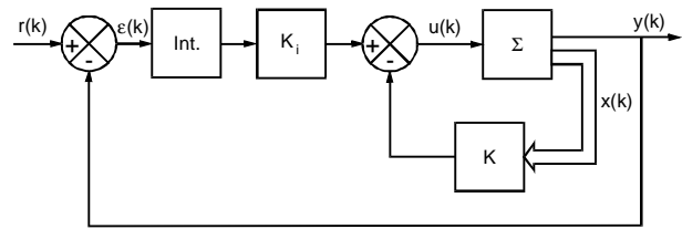
Fig. 3. State space controller
