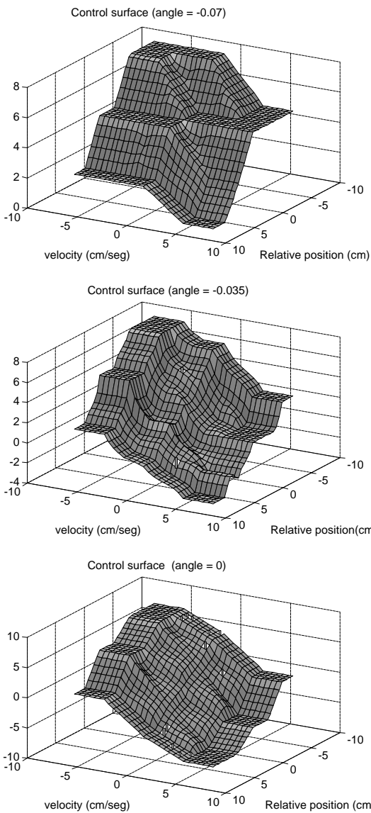
Fig. 6. Control surfaces for some negative angle positions of the bar. The case of positive angles keeps symmetry.
