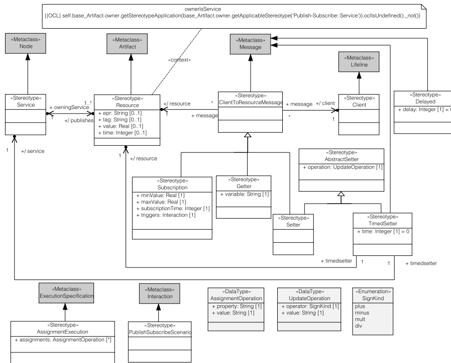
Fig. 4 UML profile for Publish/Subscribe paradigm.
