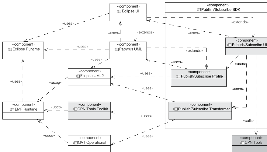
Fig. 14 Architecture of the Publish/Subscribe Modelling and Simulation Tool.
