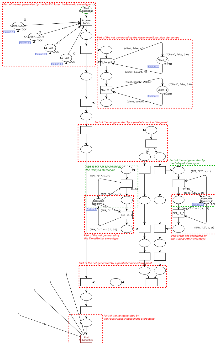
Fig. 9 Running example: TCPN model of UML-SD depicted in Figure 8.
