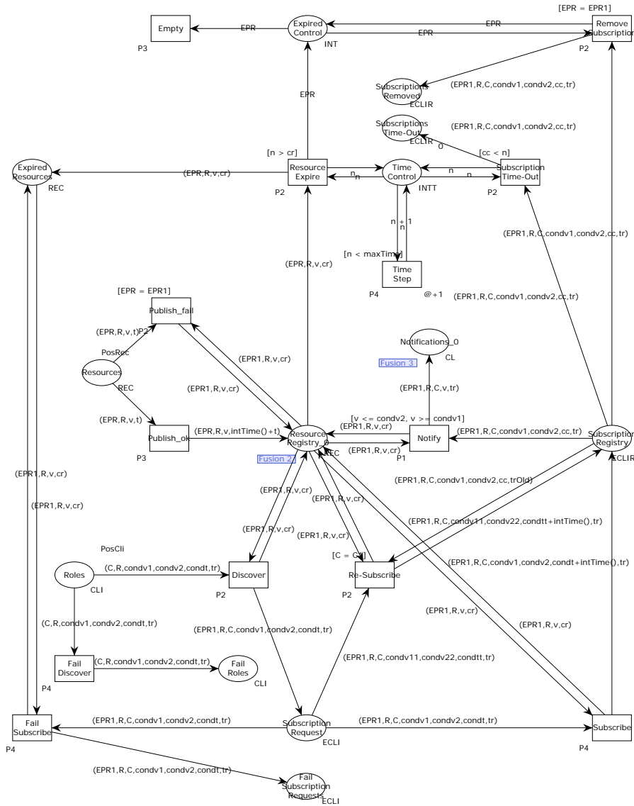
Fig. 6 Timed Colored Petri net of the PS core model (simplified with regard to (Valero et al, 2015)).
