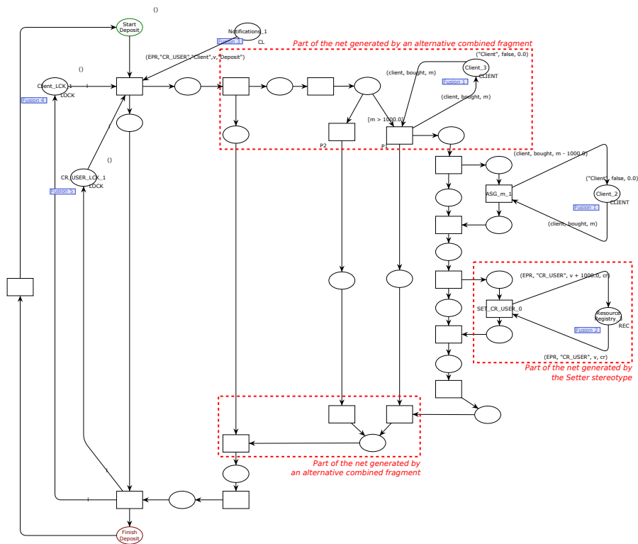
Fig. 11 Running example: TCPN model of UML-SD depicted in Figure 10.
