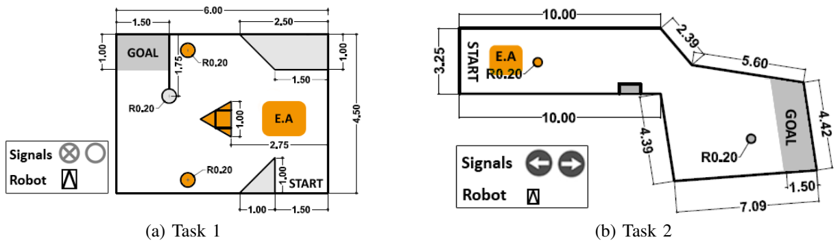
Fig. 6. (a) The objective of Task 1 was to drive the robot from the start location to the goal area. In the exploration area (E.A. in the figure), the subject had to search for two signals located in the yellow cylinders 2.5m above the floor. Then, if both signals were equal, the subject had to avoid the yellow triangle by turning to the right-hand side, or if otherwise, by turning to the left-hand side. (b) The objective of Task 2 was to drive the robot from the start location to the goal area. In the exploration area, the subject had to search for one signal located in the yellow cylinder 2.5m above the floor. The subject then had to continue navigation to the right or left direction of the two cylinders, as specified by the signal. All measures are in meters and the robot is to scale.
