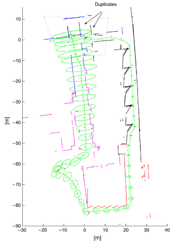
Fig. 4. Robocentric map joining before loop closing. In this case, the vehicle location uncertainty is consistent with the real error, as observed in the top left part of the figure (Note that results have been transformed back to the absolute representation).
