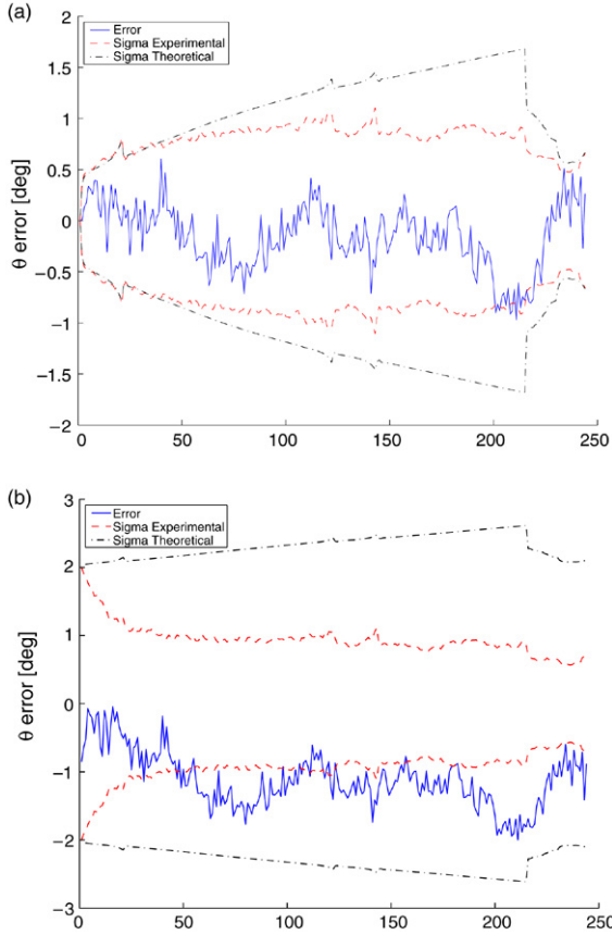
Fig. 1. Angular error and 2\sigma uncertainty bounds of the vehicle estimated location for the cases of zero (a) and nonzero (b) initial uncertainty.
