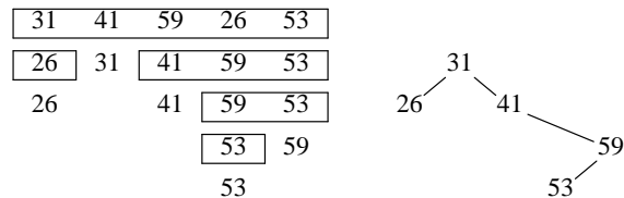
Figure 1. Quicksort and a binary search tree
