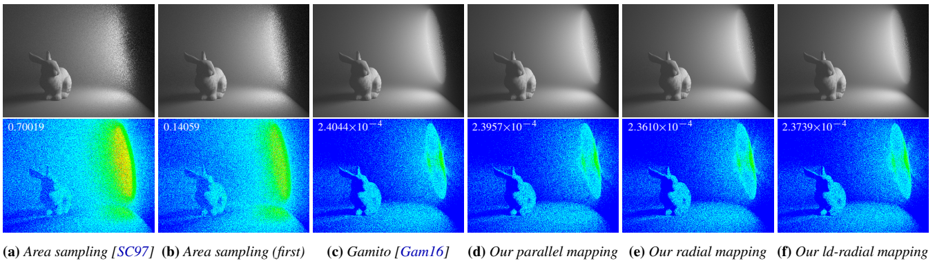
Figure 8: Top: A scene with a participating medium illuminated by a single-sided disk light (invisible), rendered with 16 samples/pixel. Please refer to Section 5 for details. Bottom: False-color differences and MSE w.r.t. to a reference image computed with 64K samples/pixel.
