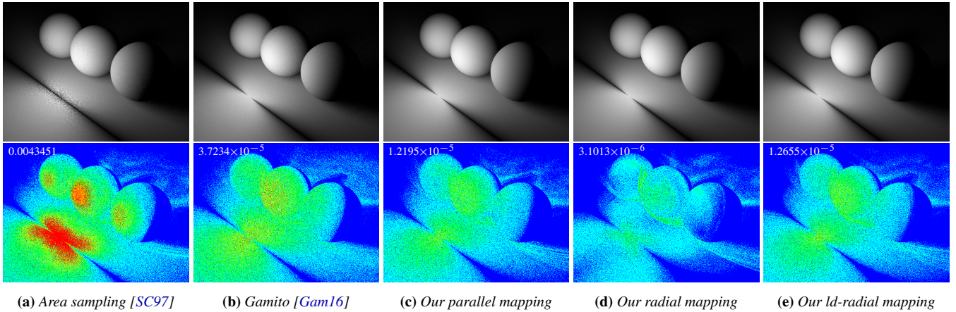
Figure 7: Top: Scene illuminated by a double-sided disk light, rendered with 16 samples/pixel. The light is perpendicular to the ground and is invisible to camera rays. Bottom: False-color differences and MSE w.r.t. to a reference image computed with 32K samples/pixel.
