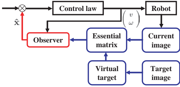
Fig. 1. Overview of the control loop. Image features are extracted and matched between the image taken at the current location and the virtual target image. The essential matrix is then estimated from the set of matches. The observer estimates the state of the system and the control law gives the velocities that lead the robot to the target location.
