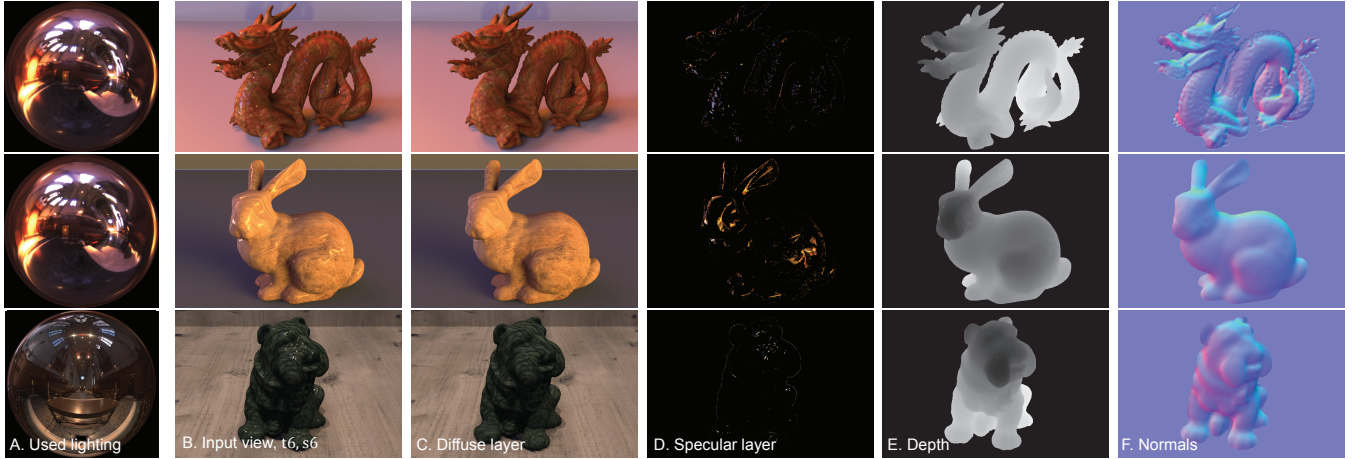
Figure 7: Steps of our preprocessing pipeline for three sample scenes: bunny, dragon and dog. All three input LFs have 11 by 11 views. For the bunny scene the disparity range is set to [-6:-3.3] , for the dragon scene to [-6:-2.5] and for the dog scene to [-5.8:-2.5] .
