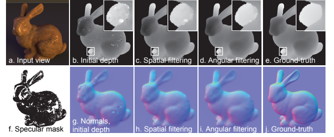
Figure 3: Illustration of the depth maps for each of the steps in Sec. 3.1. The input LF consists of 15 \times 15 views. The second row shows our estimated mask of the specular regions and the normal maps, computed as in Sec. 3.2. The maps show the values in the masked region, but the masks are not used for the steps in Sec. 3.
