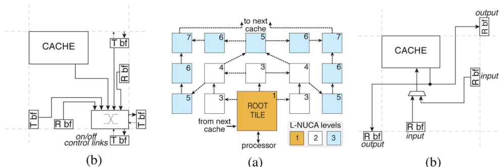
Fig. 5. Transport network topology and its components. (a) 2-D mesh topology. (b) Components.
