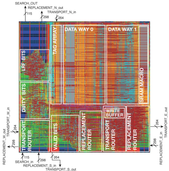
Fig. 7. L-NUCA tile layout with pin placement.
