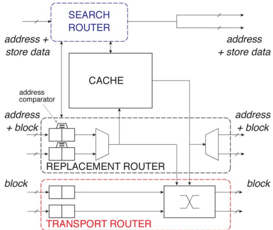
Fig. 2. L-NUCA tile main components.
