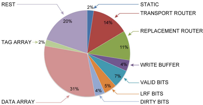
Fig. 9. Statistical power distribution.
