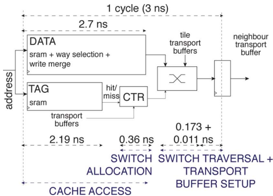
Fig. 10. Tile critical path.
