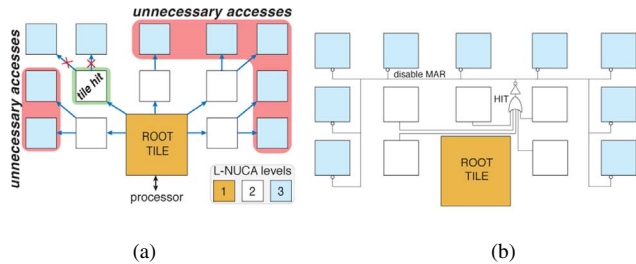
Fig. 12. L-NUCA unnecessary accesses after a second level hit and LP-NUCA with a level-2 hit detection gate. (a) Extra accesses in the third level. (b) Hit detection gate between the second and third levels.
