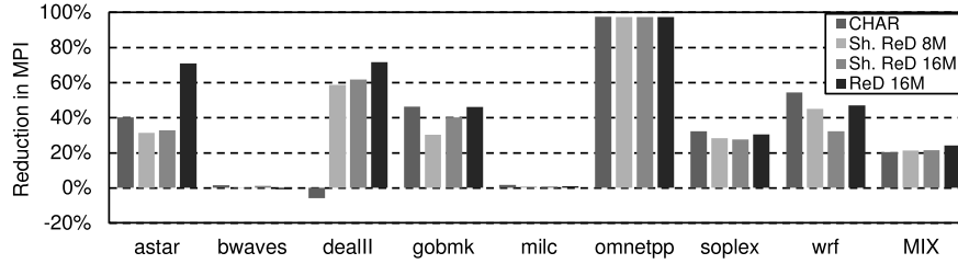
Fig. 14. SLLC MPI reduction with respect to the base system. From left to right: CHAR, Shared ReD (8 MB and 16 MB) and ReD (16 MB, 2 MB per core).
