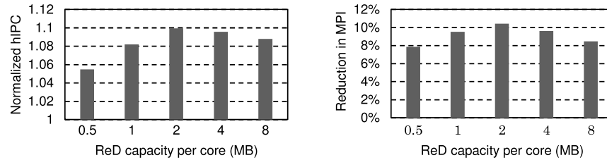
Fig. 19. Normalized hIPC (left) and reduction of SLLC misses per instruction (right) with respect to the base system, as a function of the ReD capacity per core.
