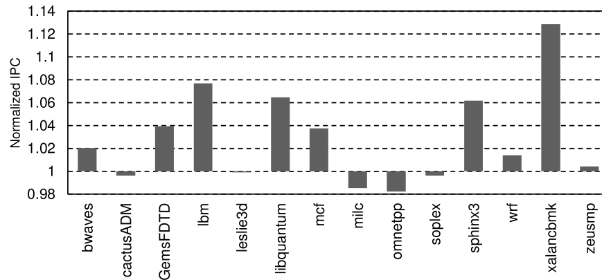
Fig. 11. Normalized IPC obtained by ReD, compared to the base system, for single-processor workloads that have LLC MPKI >2, on an exclusive LLC with 1 MB in the data array.
