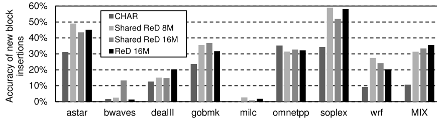
Fig. 13. Accuracy of content selection mechanisms: percentage of new blocks used at least once after being sent to the SLLC, in the example workload. From left to right: CHAR, Shared ReD (8 MB and 16 MB) and ReD (16 MB, 2 MB per core).
