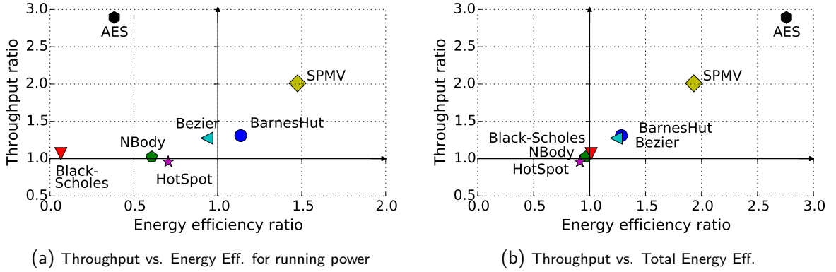
Figure 9: Throughput ratio (FPGA+2CORE to FPGA-only) vs Energy efficiency ratio (FPGA+2CORE to FPGA-only) for all the benchmarks when HAP scheduler is invoked.
