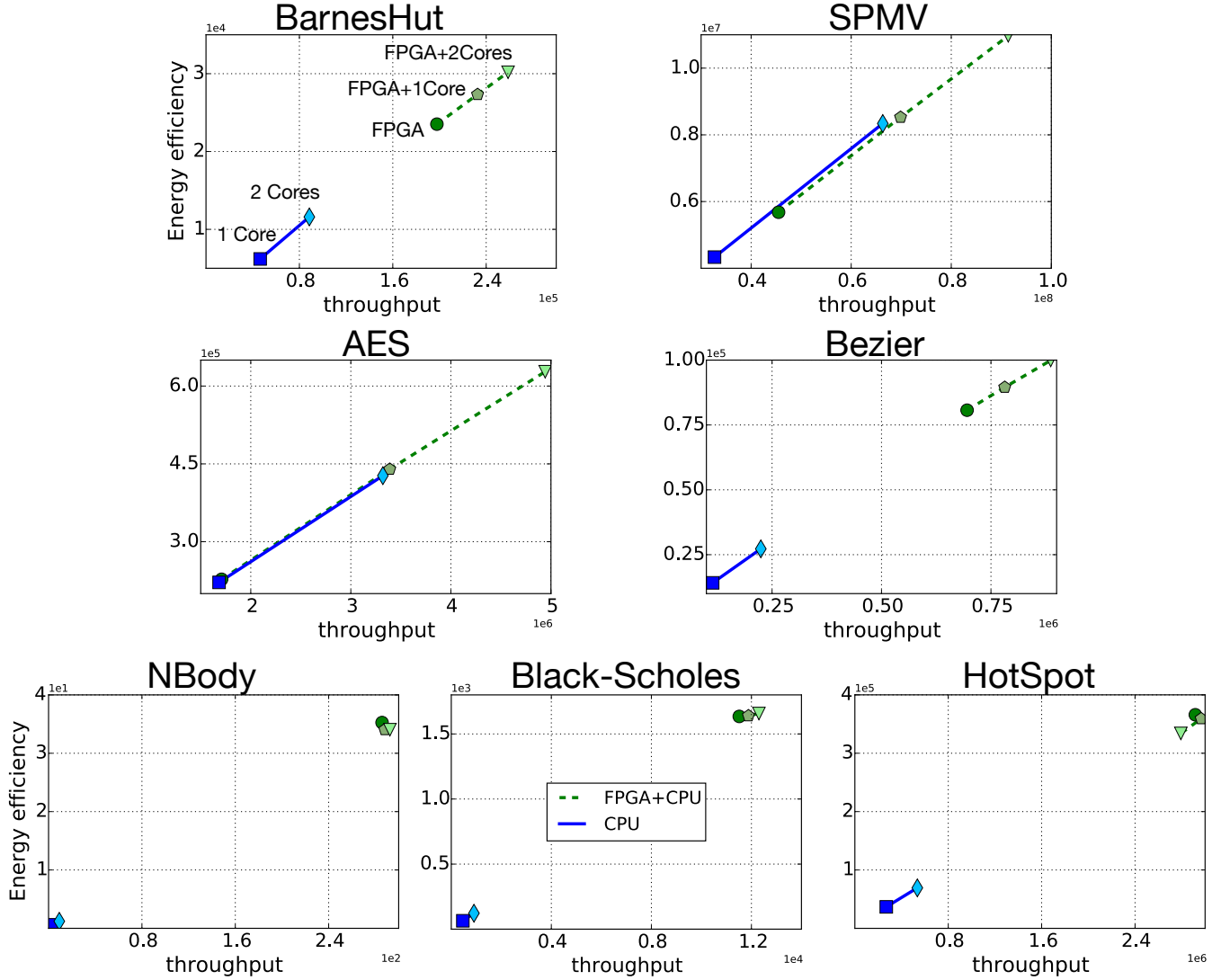
Figure 10: Efficiency-Performance plots for all benchmarks when HAP is invoked. Energy due to total power is accounted vs throughput. The higher the better in both dimensions. Throughput units are the same as in Figure 5. Energy efficiency is throughput per Watt.
