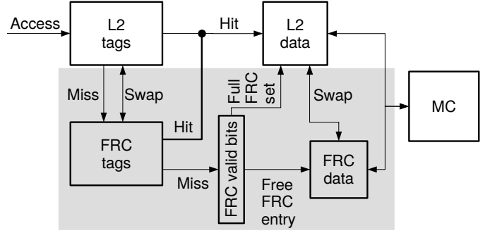
Fig. 5. FRC hardware block diagram.
