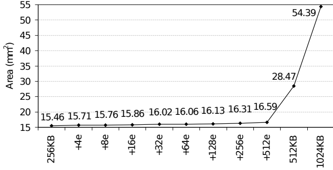
Fig. 14. Area (in \text{mm}^2 ) of the cache configurations for the RX570 GPU.
