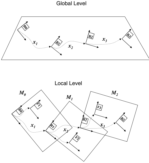
Fig. 1. Two level hierarchical SLAM model.
