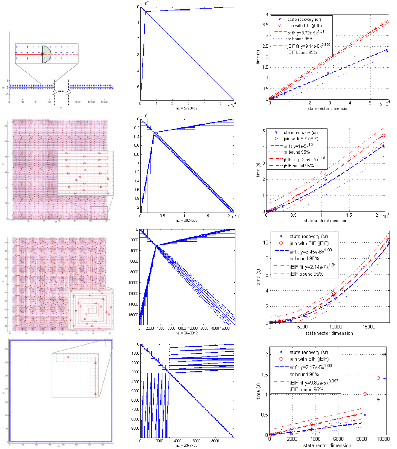
Fig. 3. Computational cost of state recovery in four cases: exploration with 27651 features (top), lawn mowing with 9056 features (upper middle), out-ward spiral with 7423 features (lower middle), several loops with 3456 features (bottom), all from 1024 local maps. From left to right: ground truth enviroment and trajectory, sparse information matrix obtained by our algorithm and execution time for to do joining and recovery state versus the state vector's dimension with their fit functions. In order to concentrate in studying computational costs these simulations were carried out with noise equal to zero.
