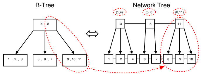
Fig. 1. Differences between B-Tree and network tree.
