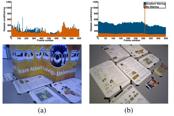
Figure 7: Hessien conditioning with and without filtering of the inverse depth gradient map in visual odometry with geometric error minimisation only in (left) structurally rich sequence and (right) structurally poor sequence.
