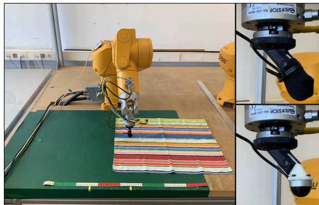
Fig. 1. Setup: A Stäubli robot arm with detail of the fingertip touch sensor covered with a silk cover at the top-right, without the cover at the bottom-right.
