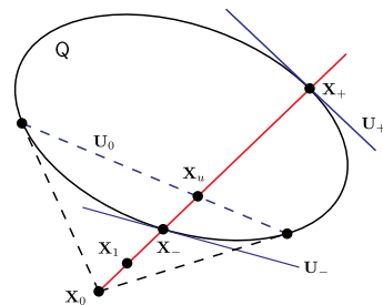
Fig. A.24. Section of a quadric. In red a 3D line intersecting the quadric. In Blue, the tangential planes U_{\pm} and the polar plane U_0 .
